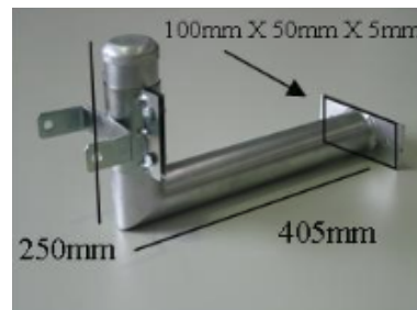
EXTENDED WALL MOUNT BRACKET (MIRROR B-E WALL)
