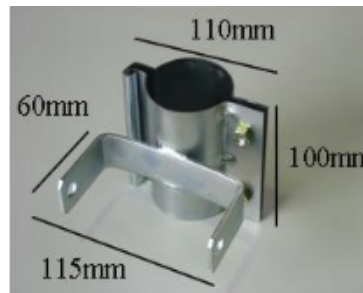
POST MOUNT BRACKET (MIRROR B- POST)
